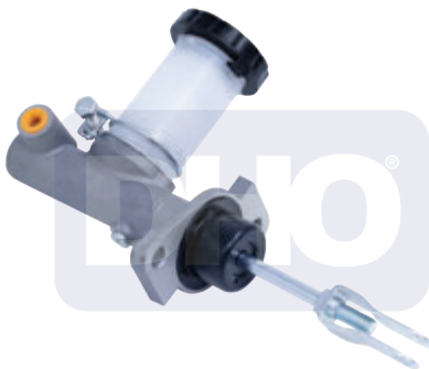
BOMBA DE CLUTCH SUP NISSAN 200SX (80-83), PICKUP 720 (80-86) LC350082, 30610-Q2101FP, CM131354
